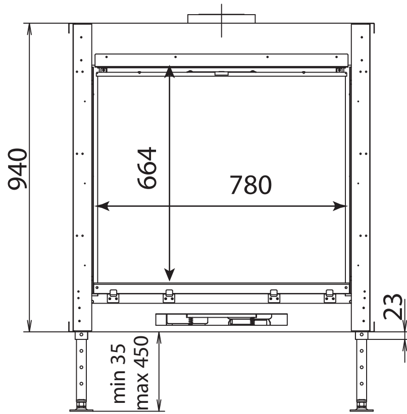
DETAIL A 1:2
